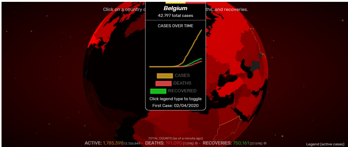
COVID-19 Visualizer
